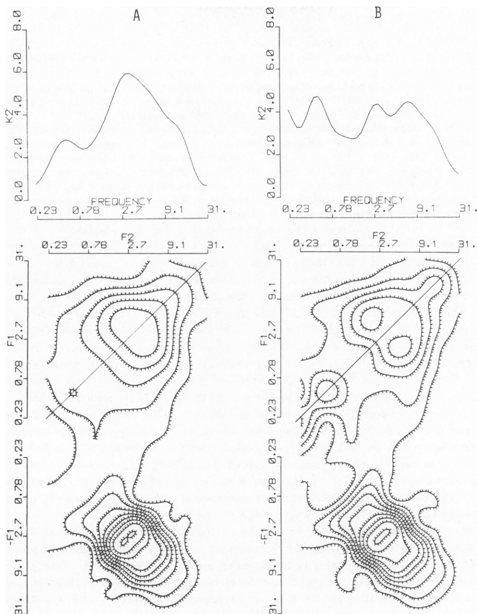
FIGURE 4 Second-order frequency kernels obtained from a cat retinal ganglion cell of the Y type. The stimulus was a 0.25 = \text{cycle/degree} grating positioned to produce no first-order response. The input signal was derived from frequency set 6, and the root-mean-squared contrast was a 0.10. Each contour line indicates 1 impulse/s; the tick marks point downhill. In (A), the algorithm to remove fourth- and sixth-order contributions was applied; in (B), this algorithm was not applied. Above each contour are plotted the second harmonic amplitudes: the values of the second-order frequency kernel along the second harmonic diagonal (where f_1 = f_2 ), which is drawn in on the contour map. The second harmonic amplitudes are plotted vs. input temporal frequency. This figure illustrates that there are irregularities near the second harmonic diagonal in (B) (without phase averaging) but not in (A) (phase-averaged). Unit 12/3.
