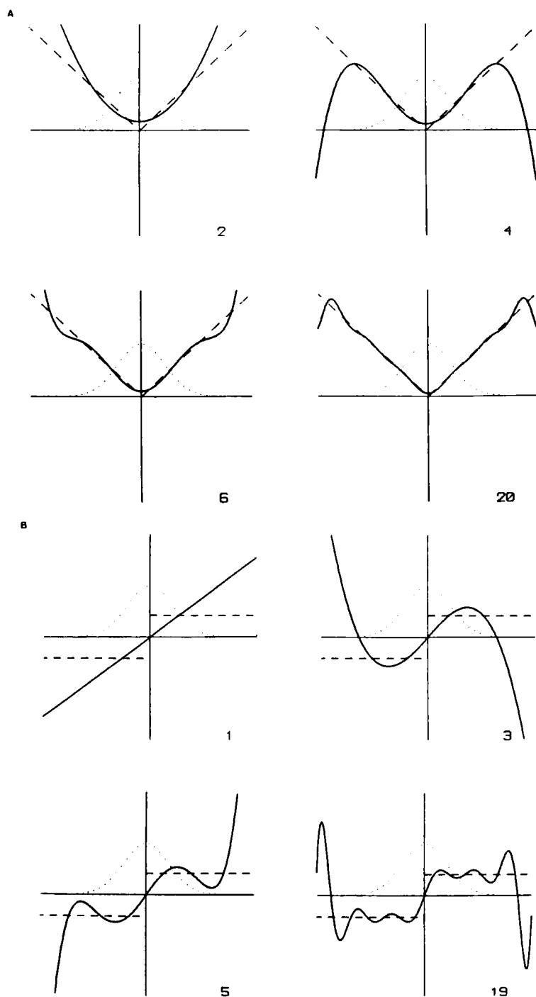
FIGURE 1 Approximation of two nonanalytic static nonlinearities by a finite sum of Hermite polynomials. In (A), approximations to the function R = |S| by second-, fourth-, sixth-, and twentieth-order polynomials are shown. In (B), the function R = \text{sgn } S is approximated by first-, third-, fifth-, and nineteenth-order polynomials.
